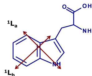
FIGURE 1. Molecular structure of tryptophan showing the transition moment directions for the transitions from the singlet ground state ( S_0 ) to the two lowest excited electronic states, ^1L_a and ^1L_b . The ^1L_a transition density is localized along the atoms (as it is directed through the ring –NH group), whereas the ^1L_b transition density lies along the bonds in the benzene ring. The change in dipole moment associated with S_0 to ^1L_a transition is larger compared to S_0 to ^1L_b transition, making the transition involving ^1L_a state more sensitive to environment. Fluorescence in most proteins arises due to ^1L_a to S_0 transition. In nonpolar environment, ^1L_a has higher energy than ^1L_b . However, the energy level of ^1L_a is lower in polar environment due to favorable dipole–dipole interactions. See text for other details. Adapted and modified from ref 17.
