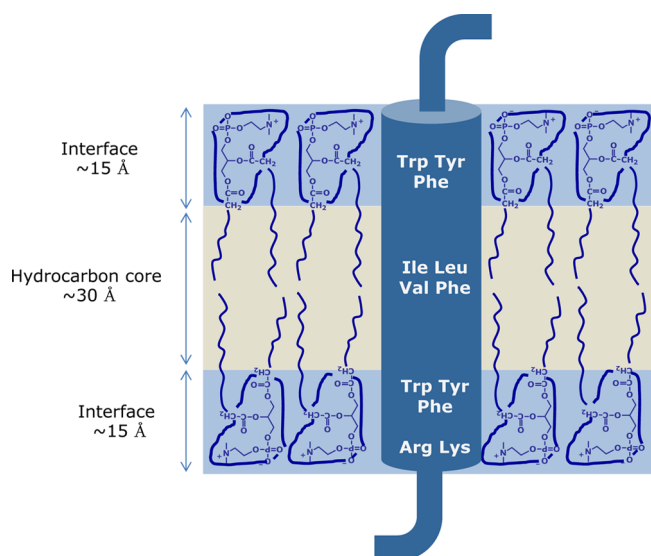
FIGURE 5. Schematic representation of biological membranes showing various regions of the bilayer with a membrane-embedded transmembrane domain. The membrane interface is represented by a heterogeneous chemical environment and relatively slow dynamics. It constitutes ~50% of the thermal thickness of the bilayer and is characterized by unique organization, dynamics, hydration and functionality. Amino acids in transmembrane helical domains display a quasi-random distribution along the bilayer normal. The preferred locations of various amino acids present in a membrane-spanning transmembrane domain are shown in the figure. It should be noted that the tryptophan residues are localized in the membrane interface region, a feature shared by many membrane proteins. 52 See text for details. Adapted and modified from ref 14.
