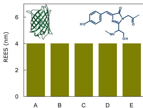
FIGURE 4. REES of the enhanced green fluorescent protein (EGFP) due to dipolar relaxation within the protein matrix is independent of bulk viscosity and dynamics. REES of EGFP in bulk water (A), glycerol (B), AOT reverse micelles of increasing hydration (C–E, corresponding to w_o = 2, 15 and 30 , respectively). The figure also shows the GFP fluorophore ( p -hydroxybenzylideneimidazolidinone) and the \beta -barrel structure of GFP. The observed REES of EGFP is due to the constrained environment experienced by the EGFP fluorophore in the rigid protein matrix, rather than the dynamics of the surrounding medium, and therefore independent of the viscosity of the medium. See ref 16 and text for details. Adapted and modified from ref 45. Copyright 2012 Springer.
