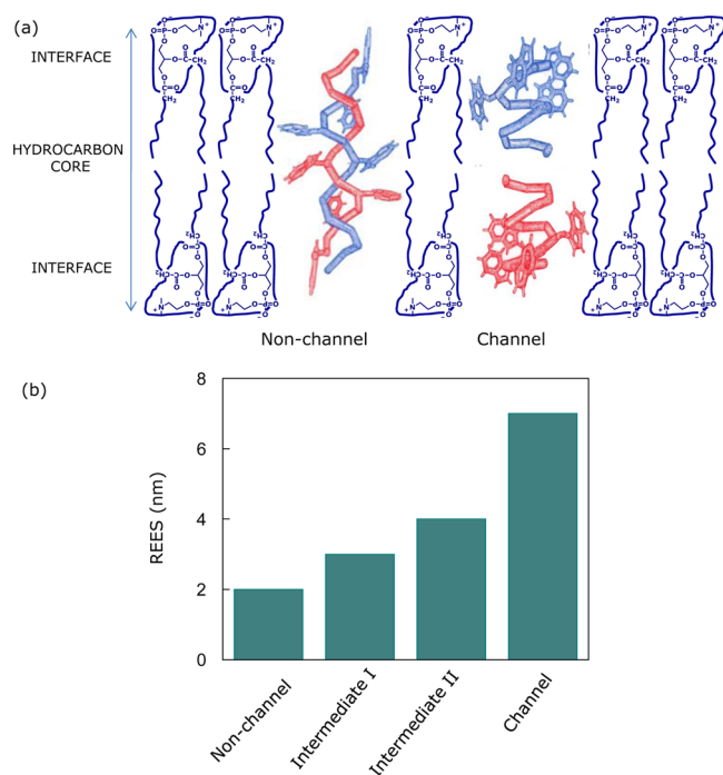
FIGURE 6. Conformation-dependent REES of membrane proteins. (a) A schematic representation of the non-channel and channel conformations of the ion channel peptide gramicidin indicating the localization of tryptophan residues in the membrane bilayer. Tryptophan residues are clustered toward the membrane interface in the channel conformation, whereas they are distributed along the membrane z axis (bilayer normal) in the non-channel conformation. Gramicidin is a popular membrane peptide and is extensively used to explore the principles that govern the folding and function of membrane proteins (see ref 64). Adapted with permission from ref 15. Copyright 2011 American Chemical Society. (b) REES is sensitive to the conformation of membrane-bound gramicidin. Intermediates I and II represent intermediates in the folding pathway of the channel conformation from non-channel conformation. The magnitude of REES corresponds to the total shift in emission maximum as the excitation wavelength was changed from 280 to 307 nm. Data from ref 61.
