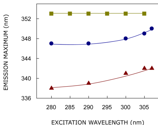
FIGURE 2. Detection of local residual structure by REES. Effect of changing excitation wavelength on the wavelength of maximum emission of the cytoskeletal protein spectrin in native (▲) and denatured (●) conditions. Tryptophan residues in denatured proteins usually do not display REES since they are exposed to bulk water (the figure also shows lack of REES in a representative denatured protein, tubulin (■)). The presence of REES in denatured spectrin therefore demonstrates that spectrin tryptophans are shielded from bulk water even when denatured, thereby implying local residual structure in denatured spectrin. The residual structural integrity that remains in denatured spectrin is considered to be the hallmark of a protein whose main function is to provide a stable scaffold to the cell membrane. See text for details. Data from refs 24 and 26.
