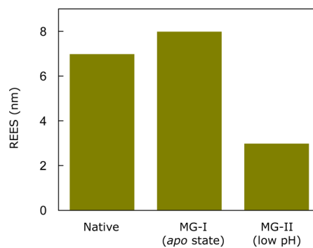
FIGURE 3. Protein conformations and REES: REES exhibited by tryptophan residues of bovine \alpha -lactalbumin (BLA) in native and molten globule states. MG-I refers to the \text{Ca}^{2+} -depleted ( apo -state) molten globule conformation (see ref 39) and MG-II refers to the molten globule state of BLA induced by low pH (ref 40). These results are one of the first reports of REES in molten globule conformation of proteins. Note that the magnitude of REES appears to depend on the manner in which the molten globule state was achieved, indicating that the molten globule states represent an ensemble of conformations with varying degrees of disorder. The magnitude of REES corresponds to the total shift in emission maximum as the excitation wavelength was changed from 280 to 307 nm. See text and refs 39 and 40 for details.
